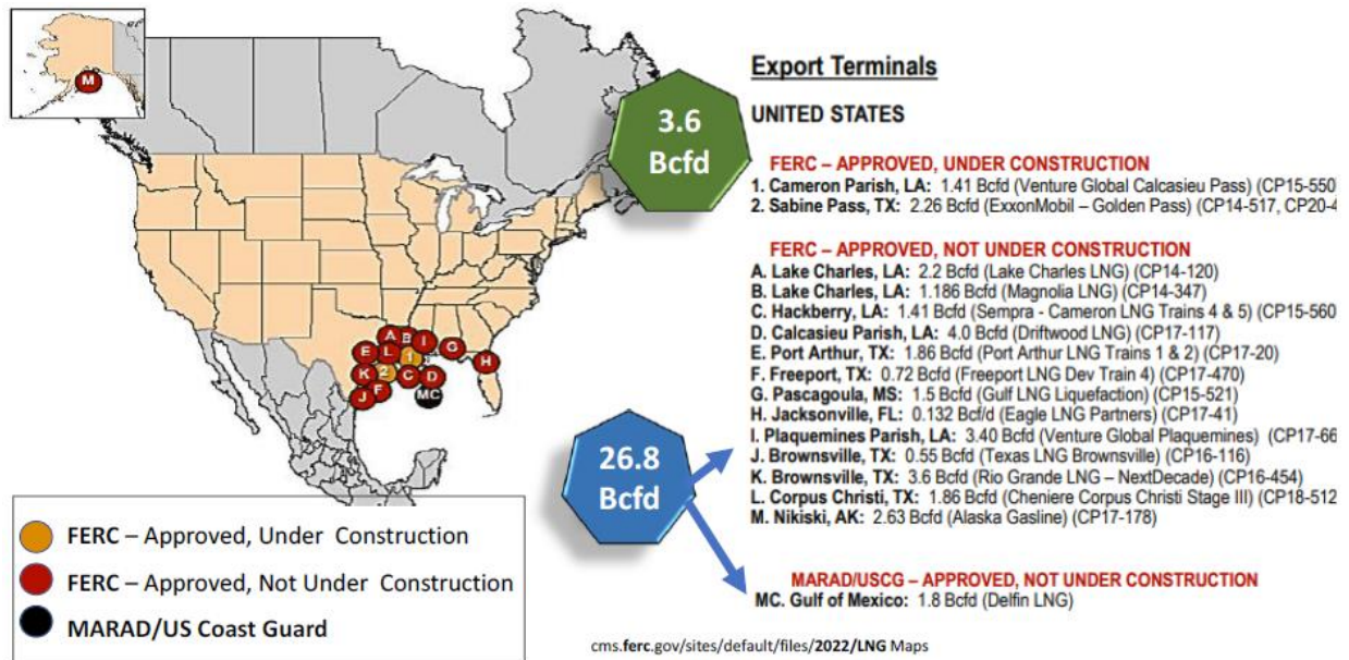
Figure 3. Approved US LNG Export Terminals as of 2/16/2022
