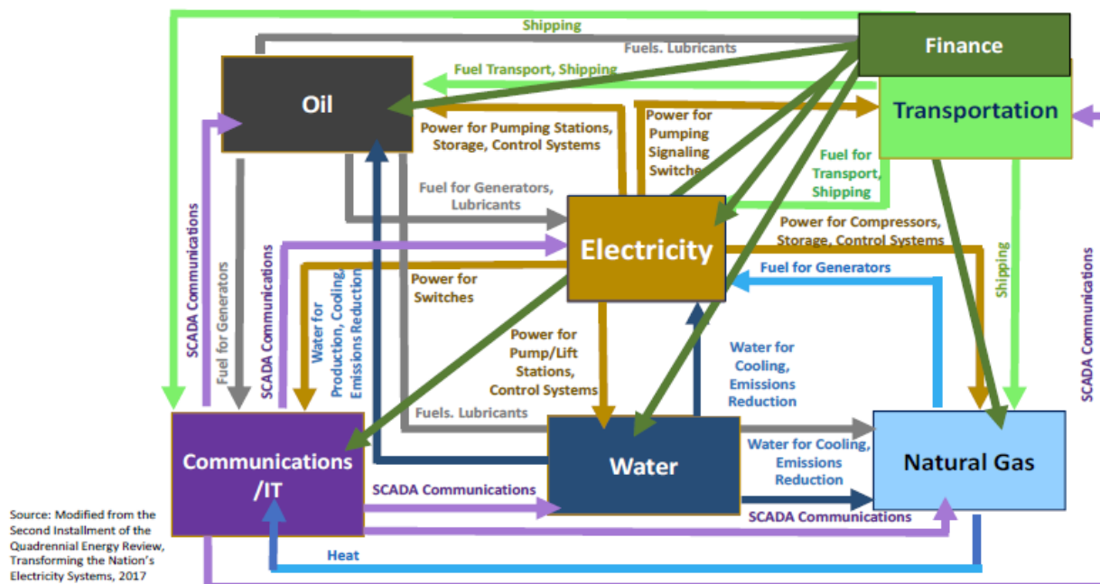
Figure 6. Electricity and Lifeline Network Interdependencies
