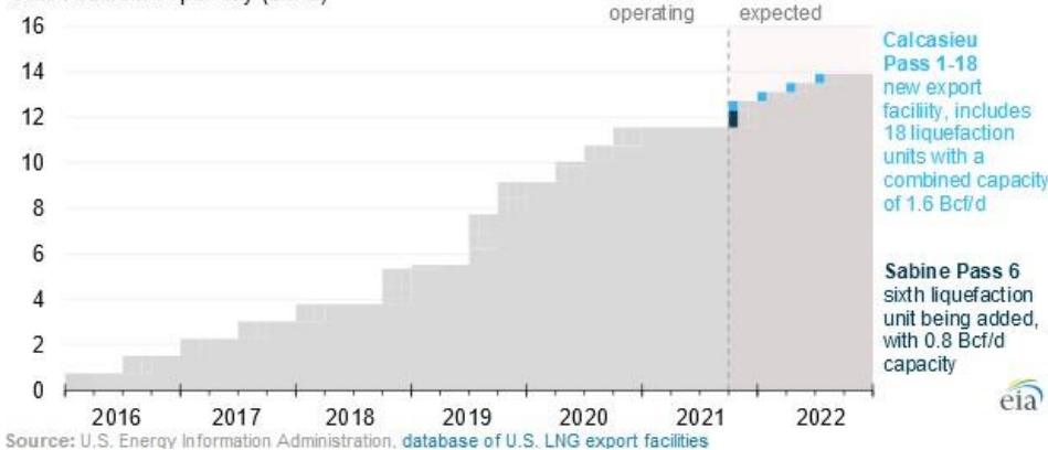
Figure 2. US Liquefied Natural Gas Export Capacity Largest in the World in 2022
